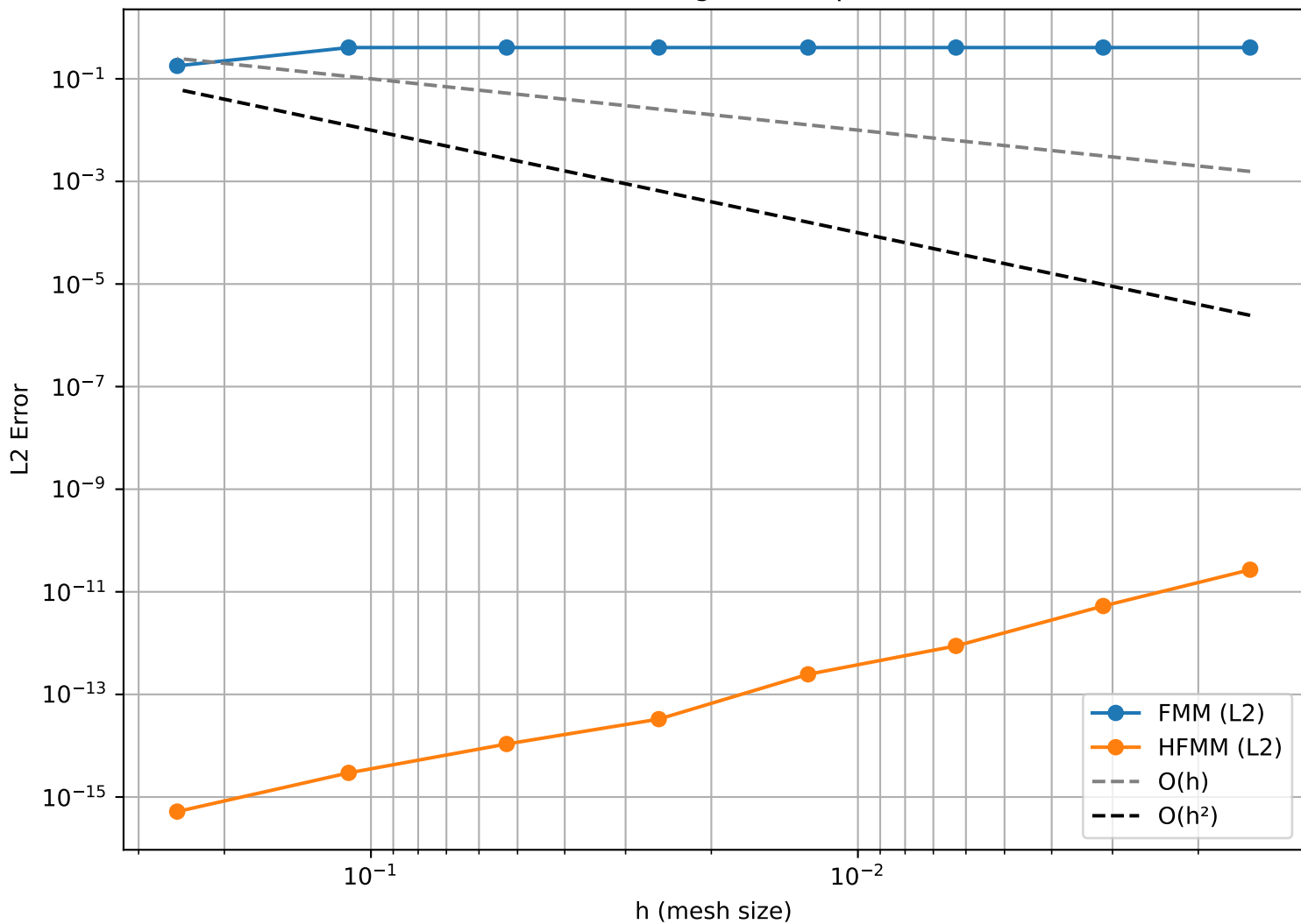
FMM Convergence - Square
